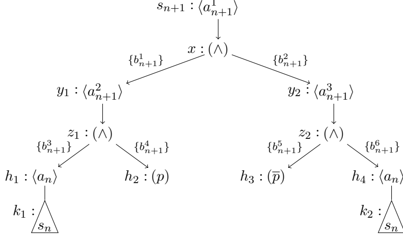
Fig. A.1. s_{n+1} , minimum uniform strategy tree winning for \mathcal{G}_{\mathcal{N}_{n+1}}^{\diamond\wedge\lrcorner}(\{a_{n+1}\}, \{b_{n+1}\}) .
