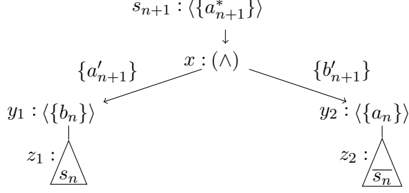
Fig. 2. s_{n+1} , minimum uniform strategy tree winning for \mathcal{G}_{\mathcal{M}_{n+1}}(\{a_{n+1}\}, \{b_{n+1}\}) .
