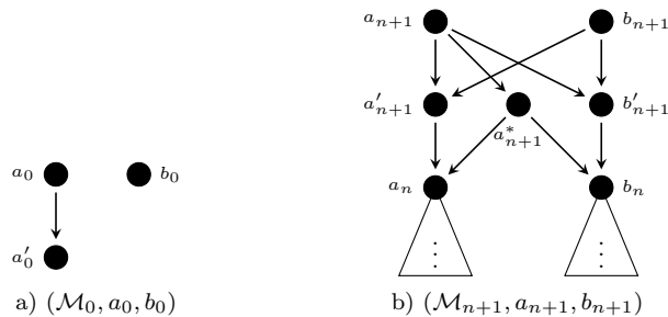
Fig. 1. Recursive family of models (\mathcal{M}_n, a_n, b_n)_{n \in \mathbb{N}}
