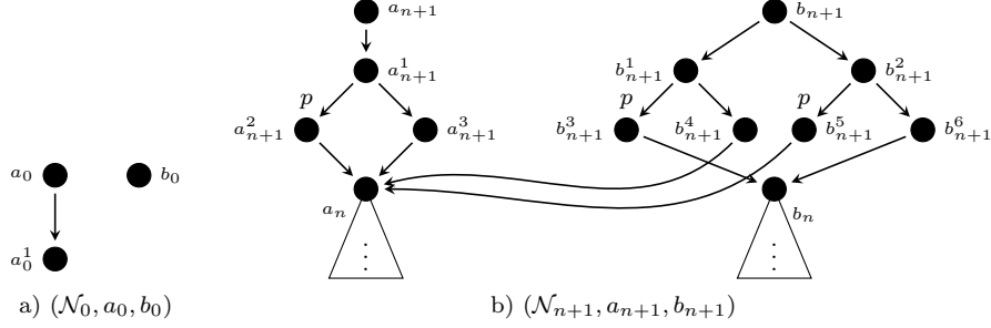
Fig. 3. Recursive family of models (\mathcal{N}_n, a_n, b_n)_{n \in \mathbb{N}}
