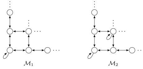
Figure 1: Two \mathcal{M}_0(\oplus, \otimes) -bisimilar models
